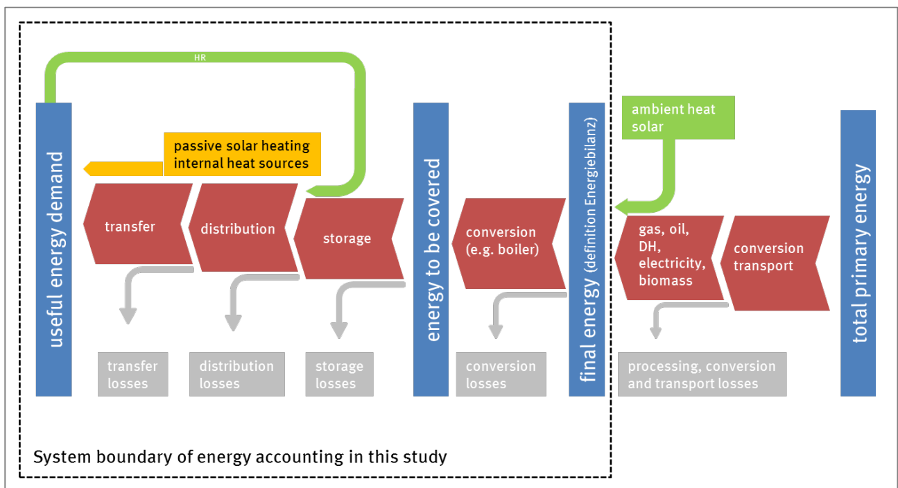
Figure I: Schematic energy flux diagram
