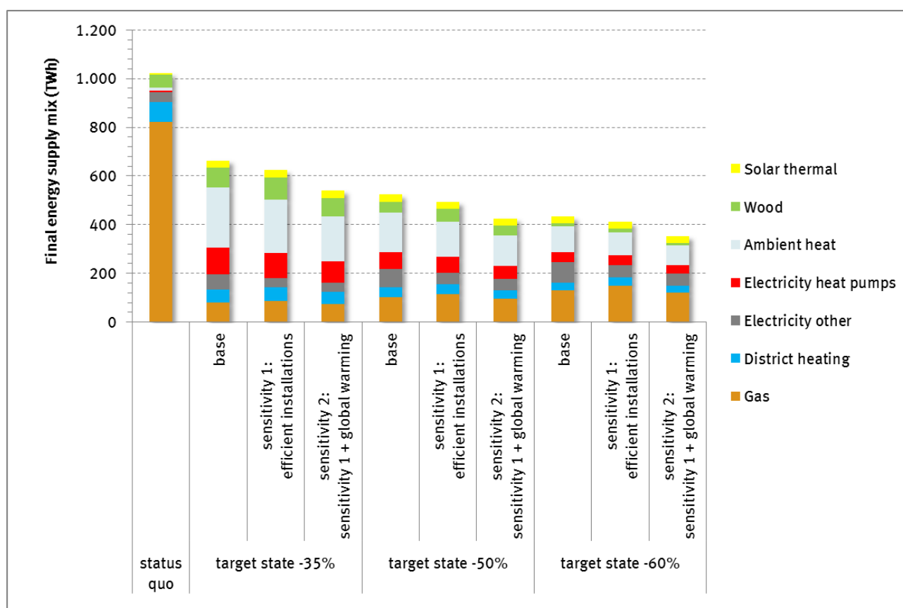
Figure IX: Final energy supply mix (according to the energy balance accounting rules) of the entire building stock for the different target states and sensitivities
