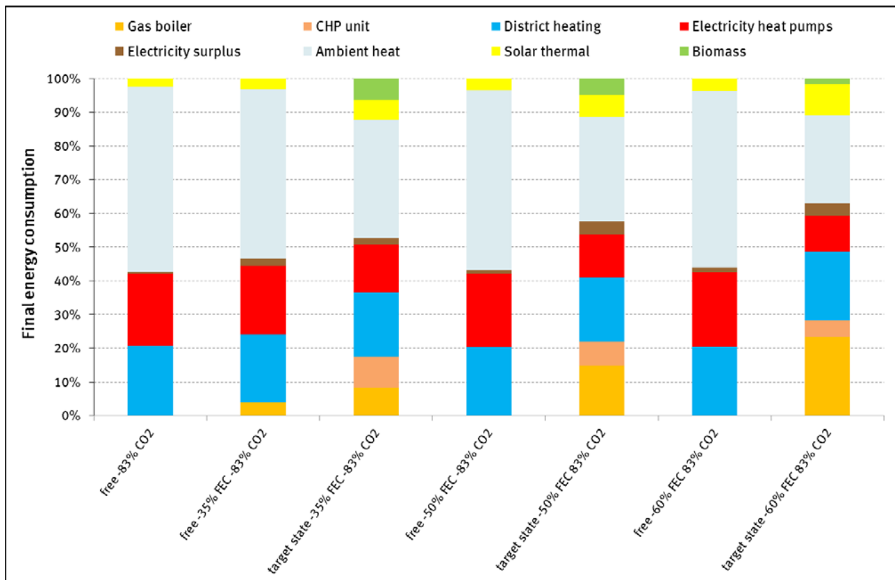
Figure VIII: Distribution of final energy consumption sources for heating in 2050 for different scenarios
