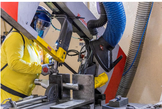
Figure D-16: Disassembly work in the residual material treatment centre of the Grafenrheinfeld nuclear power plant in the controlled area Left: Sawing centre of the residual material treatment centre in the annulus (Copyright: PreussenElektra GmbH, photographer: Johannes Kiefer) Right: Final disassembly station of the residual material treatment centre in the reactor auxiliary building (Copyright: PreussenElektra GmbH, photographer: Johannes Kiefer)
