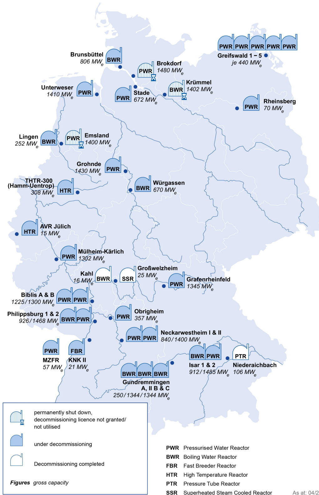
Figure A-2: Nuclear power plants, experimental and demonstration reactors in Germany
