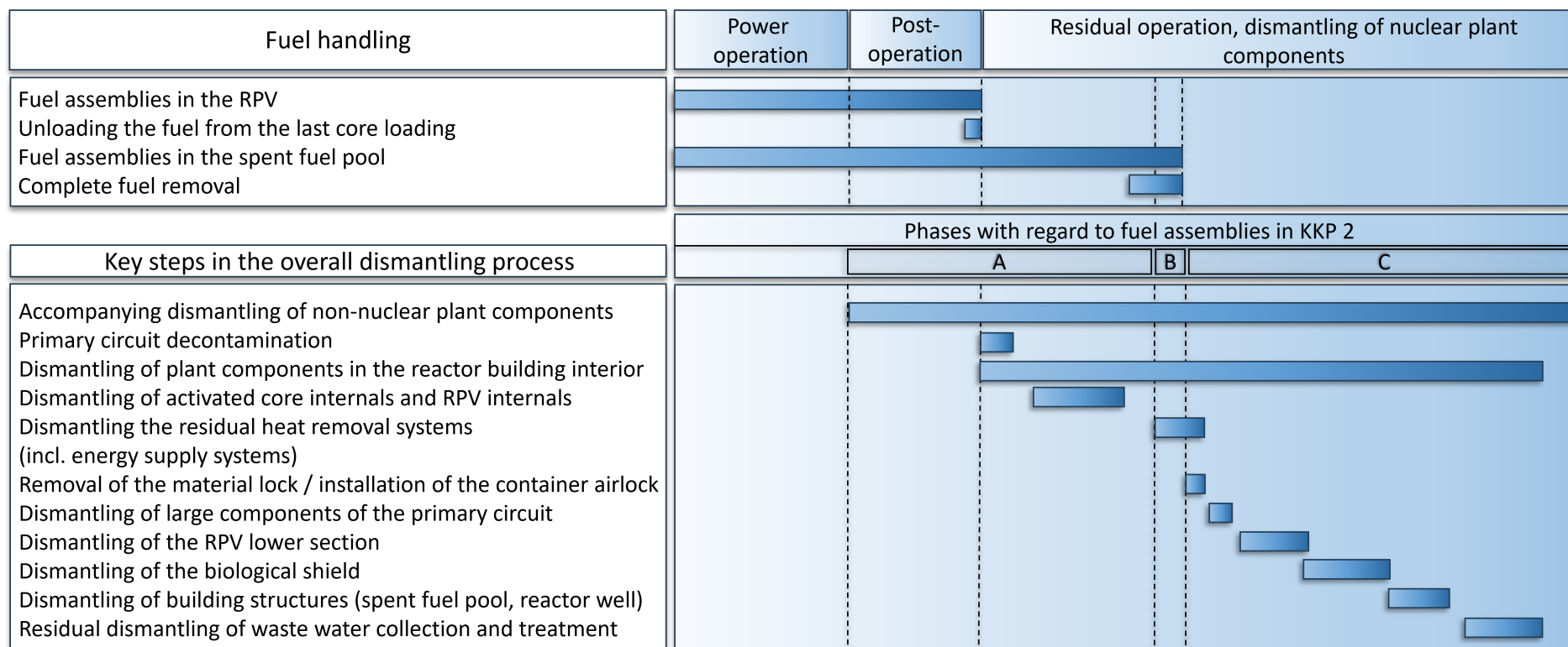
Figure D-15: Main dismantling steps in the dismantling of Unit 2 of the Philippsburg nuclear power plant within the framework of a single decommissioning and dismantling licence (planning status)
