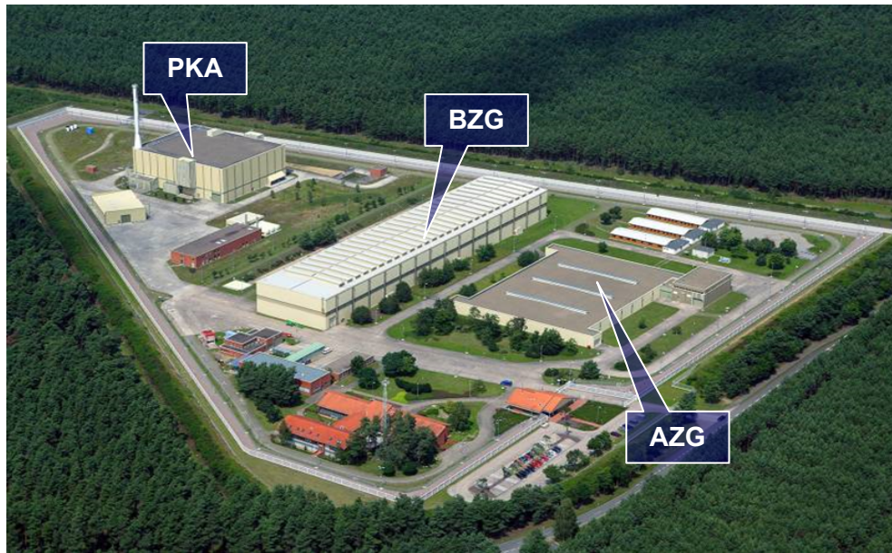
Figure D-3: View into the Gorleben spent fuel storage facility (Copyright: BGZ) Transport and storage casks of various types
